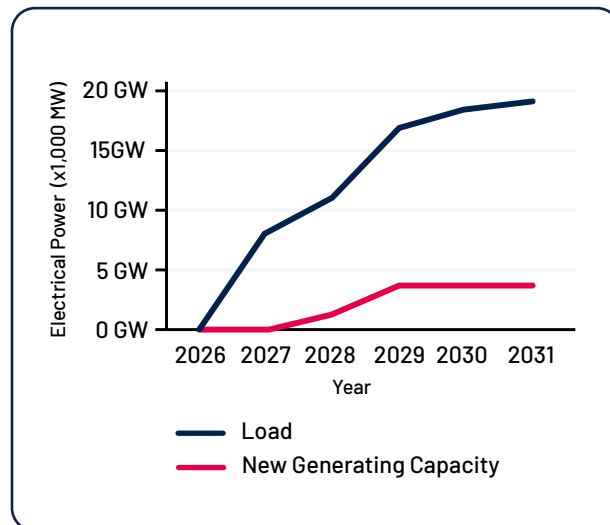
Figure 4. Alberta Data Centre Load Demand Versus New Generating Capacity
